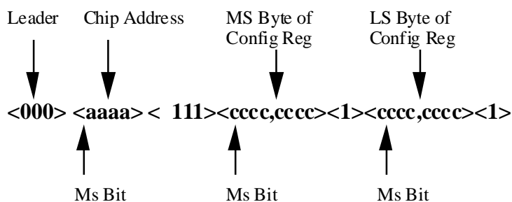
Figure 3.17e. Configuration Data Packet.
