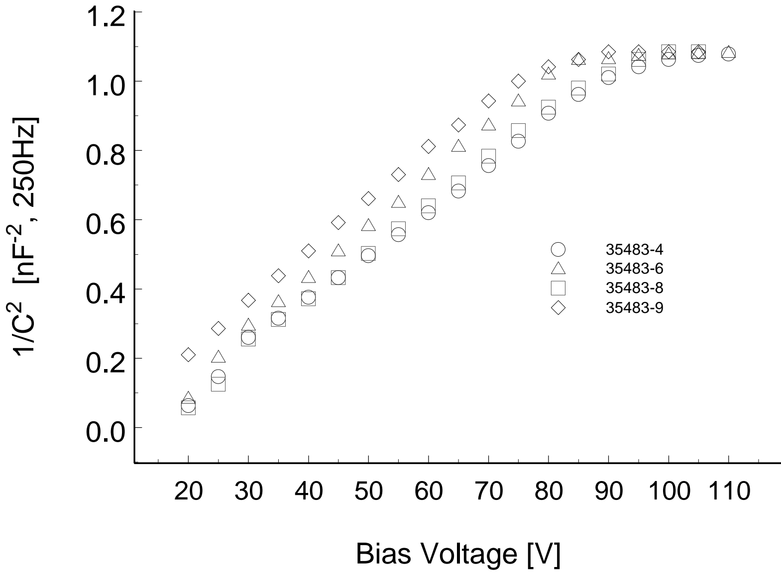
Capacitance as a Function of Bias Voltage
