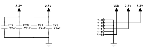
Shifter Power Filtering
