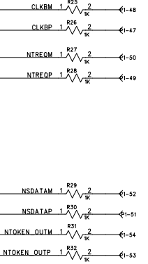
GTRC Probes Filtering
