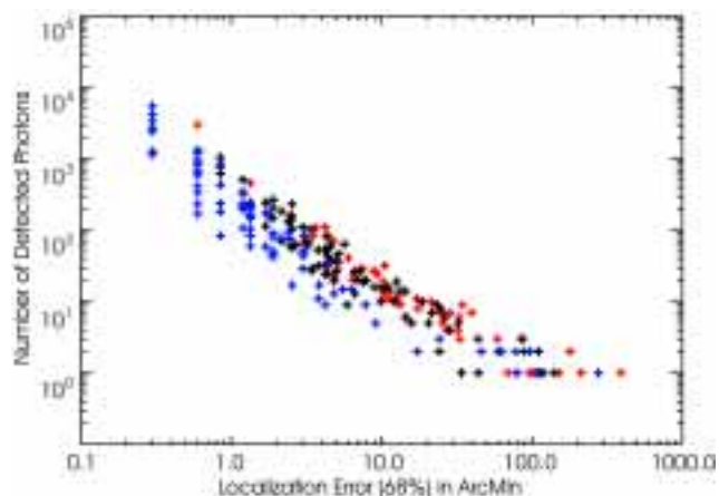
Figure 6-4 Simulation showing the accuracy of location determination for the >200 GRBs per year that will be detected by the LAT. A realistic, discrete distribution of power-law spectral indices was used, based on EGRET spark chamber and TASC detections of GRBs. The points are color coded by spectral index: blue (1.6, 1.8), black (2.0), and red (2.2, 2.4). The simulation uses flux and duration distributions determined by BATSE below 1 MeV, in addition to the power-law indices, to extrapolate the GRB fluences to energies greater than 100 MeV.
