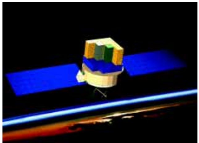
Figure 2-2 An instrument/spacecraft concept for GLAST (see §11 & 12). Some towers and part of the LAT calorimeter have been removed in this cutaway view.
