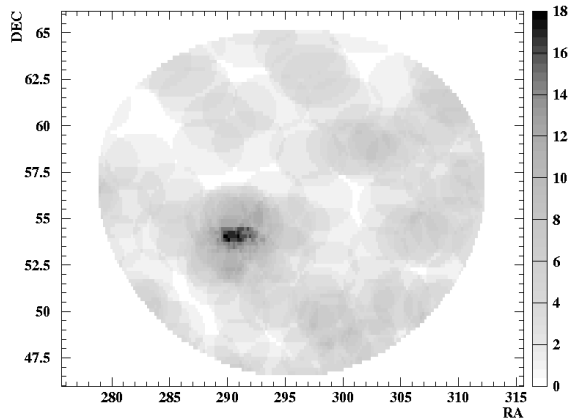
FIGURE 1. Number of events recorded by Milagrito during T90 in the BATSE 90% error radius for GRB 970417, each bin contains the number of events detected by Milagrito within a 1.6 degree radius.
