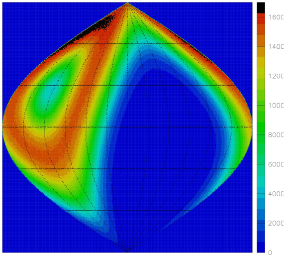
Fig. 1. The density of events from Milagro (in arbitrary units) plotted in galactic coordinate system, sine equal area projection. Grid lines are plotted every 30^\circ in longitude and latitude. Galactic center is in the middle of the map
