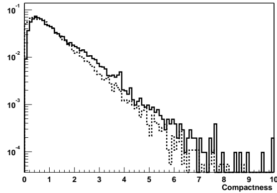
Fig. A1. The compactness distribution for Monte Carlo protons (solid line) and data using the updated calibration constants (dashed line).
