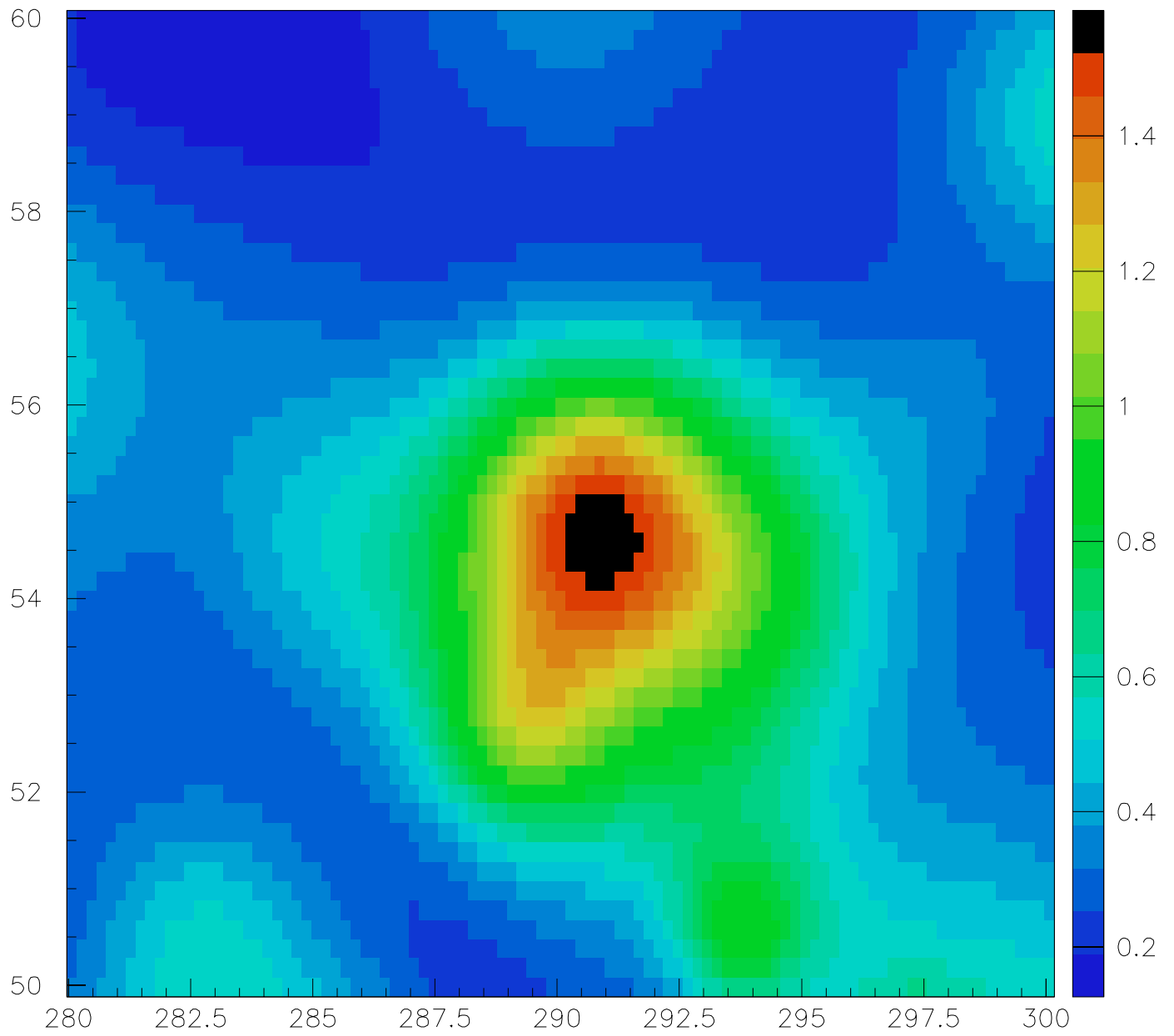
Gaussian Map Burst 1
