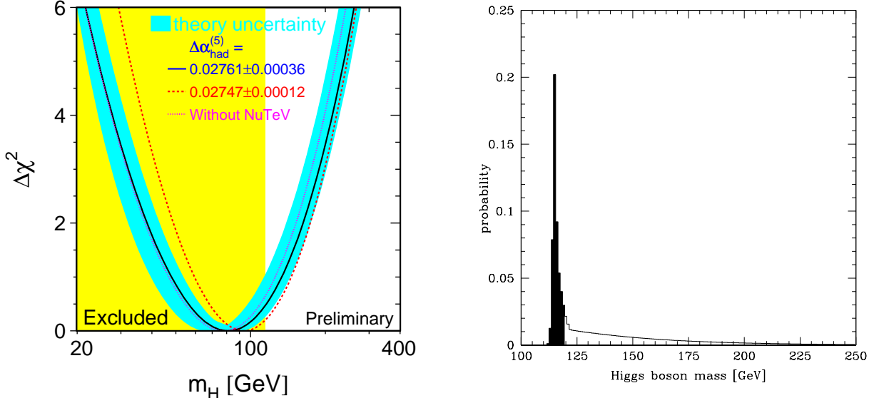
Figure 1: (a) The “blueband plot” shows \Delta\chi^2 \equiv \chi^2 - \chi_{\min}^2 as a function of the SM Higgs mass [1]. The solid line is a result of a global fit using all data; the band represents the theoretical error due to missing higher order corrections. The rectangular shaded region shows the 95% CL exclusion limit on the Higgs mass from direct searches at LEP [2]. (b) Probability distribution function for the Higgs boson mass, including all available direct and indirect data [3]. The probability is shown for 1 GeV bins. The shaded and unshaded regions each correspond to an integrated probability of 50%
