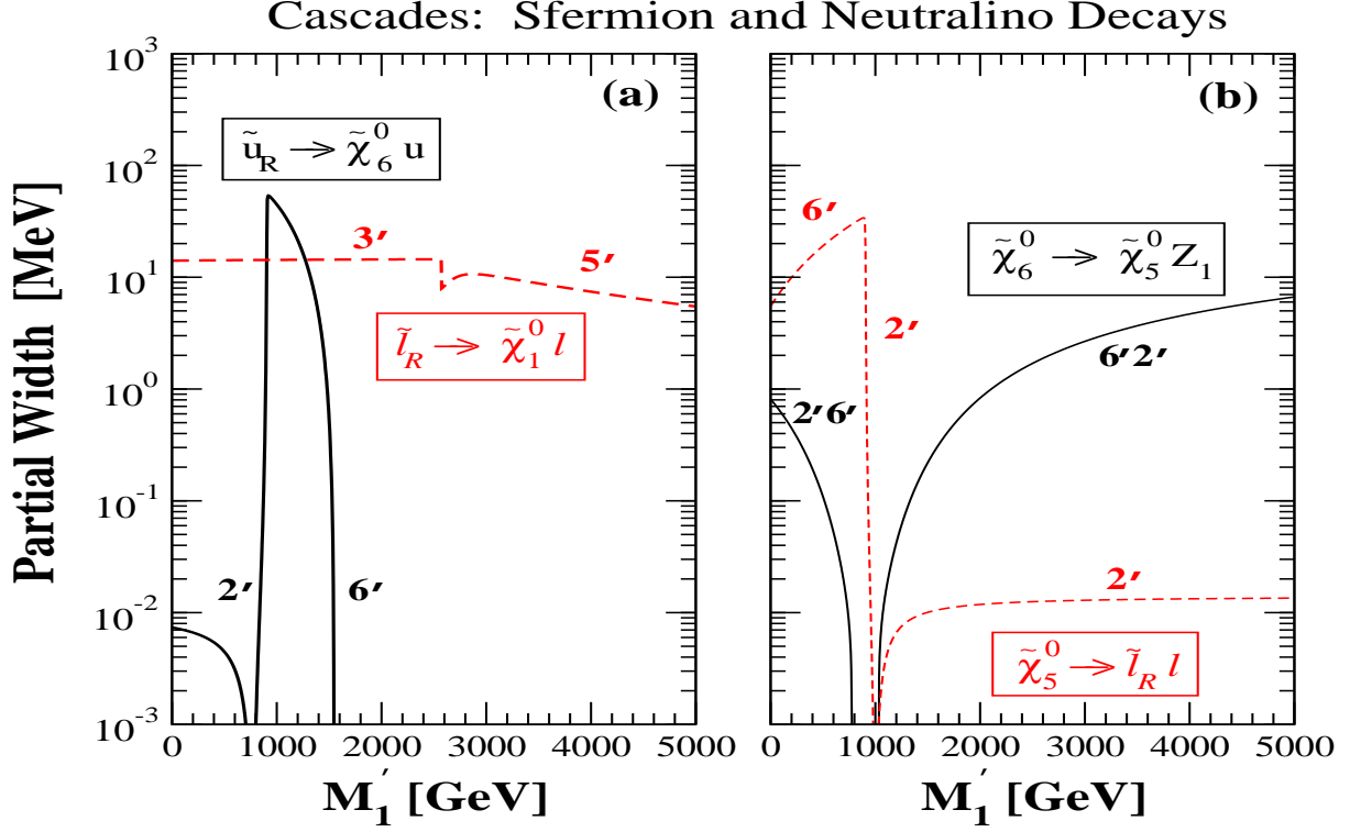
Figure 5: The evolution of (a) the sfermion decays, \tilde{u}_R \rightarrow \tilde{\chi}_6^0 u and \tilde{l}_R \rightarrow \tilde{\chi}_1^0 l , and (b) the neutralino decays, \tilde{\chi}_6^0 \rightarrow \tilde{\chi}_5^0 Z_1 and \tilde{\chi}_5^0 \rightarrow \tilde{l}_R l , when varying the U(1)_X gaugino mass parameter M'_1 . The R-type slepton and R-type u-squark masses are m_{\tilde{l}_R} = 701 GeV and m_{\tilde{u}_R} = 2000 GeV, respectively.
