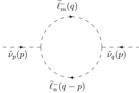
Fig. 3. Slepton pair loop contribution to the sneutrino–antisneutrino mass splitting.
