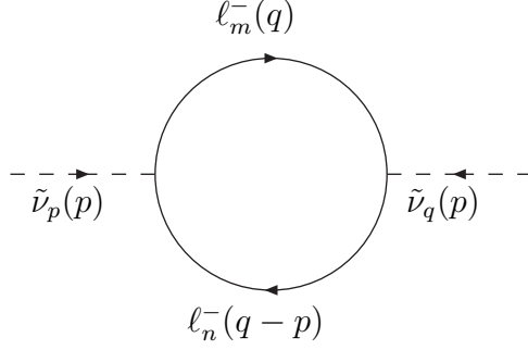
Fig. 2. Lepton pair loop contribution to the sneutrino–antisneutrino mass splitting.
