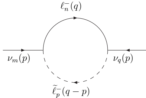
Fig. 1. One-loop contribution to the neutrino mass.
