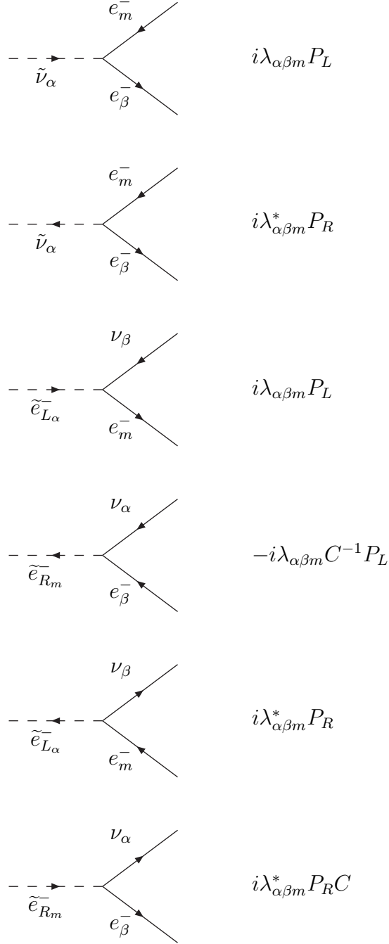
Fig. 4. Feynman rules for the scalar–fermion interactions.
