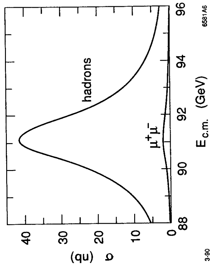
Figure 6. Total cross section for e^+e^- annihilation in the vicinity of the Z^0 , to leading order in \alpha .
