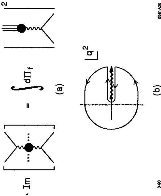
Figure 26. Evaluation of the hadronic contribution to the electromagnetic vacuum polarization.
