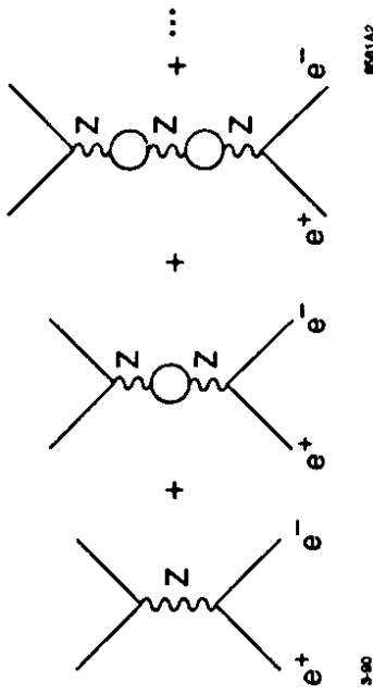
Figure 2. Feynman diagrams whose summation produces the Breit-Wigner denominator of the Z^0 propagator.
