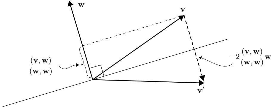
Figure 29.1: Orthogonal reflection in the hyperplane perpendicular to \mathbf{w} .
