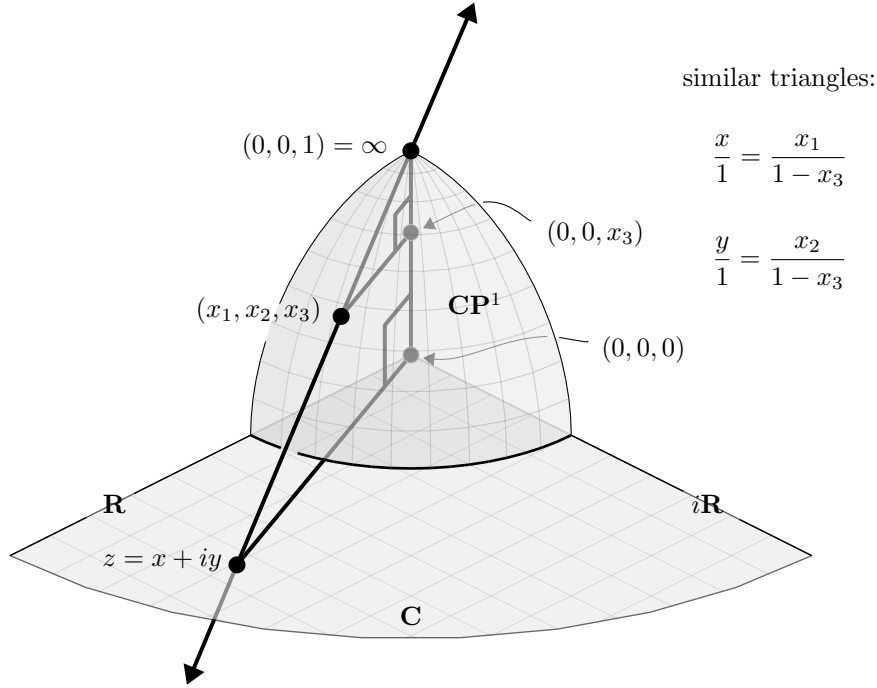
Figure 7.2: Complex-valued coordinates on \mathbf{CP}^1 - \{\infty\} via stereographic projection.
