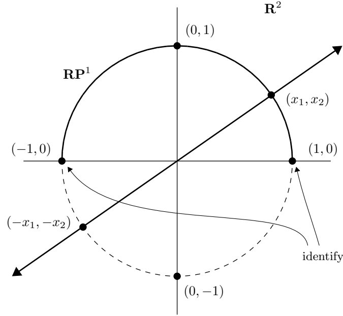
Figure 6.2: The real projective line \mathbf{RP}^1 .
