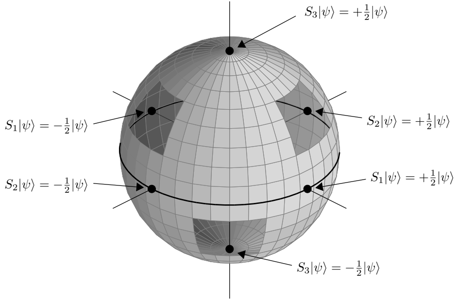
Figure 7.3: The Bloch sphere.
