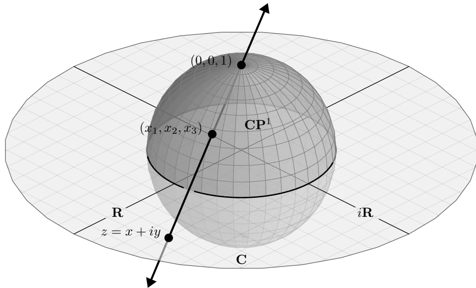
Figure 7.1: The complex projective line \mathbf{CP}^1 .
