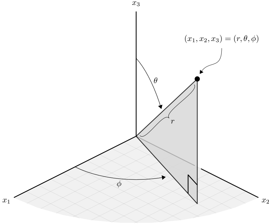
Figure 8.2: Spherical coordinates.
