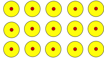
Figure 59: A simple model of a neutral material
