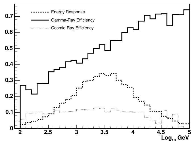
FIG. 5.—Fraction of gamma rays and cosmic rays retained by the compactness cut ( C > 2.5 ) as a function of primary energy. The dashed line (labeled “Energy Response”) shows the energy distribution of the gamma rays that trigger Milagro. The gamma rays were generated with an E^{-2.4} spectrum.
