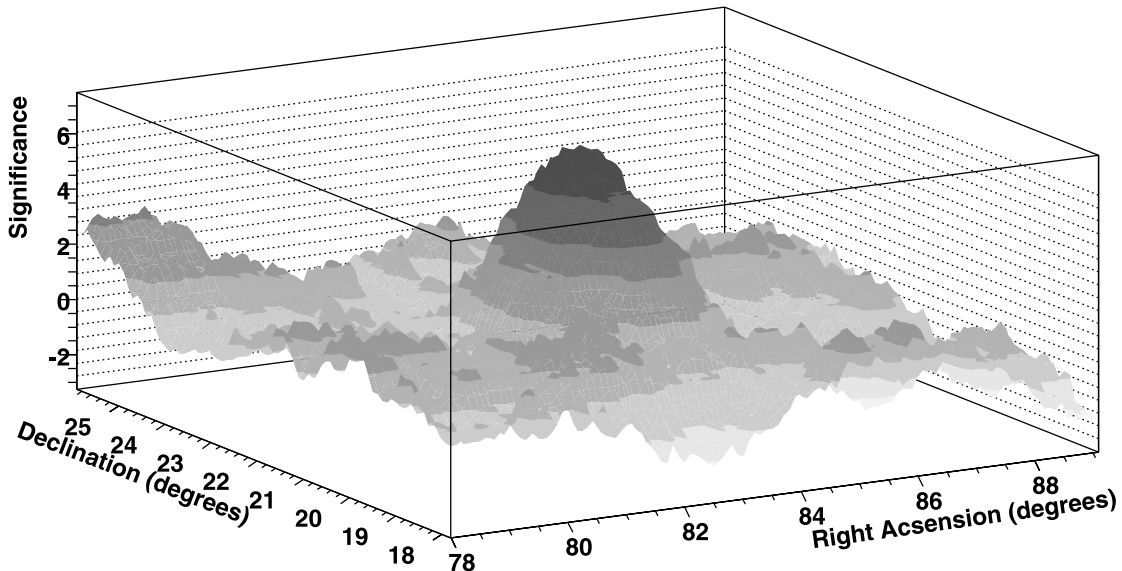
FIG. 10.—Map of the statistical significances in the region around the Crab Nebula. The z -axis is in standard deviations.
