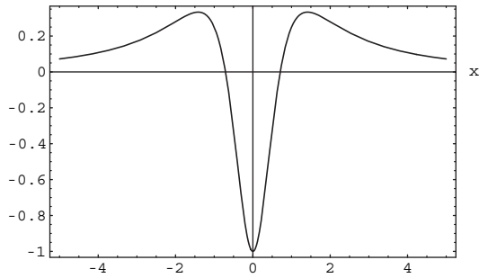
Fig. 2: The potential (V(x) - E) in eq. (13) for \gamma^2 = 0 .
