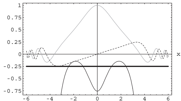
Fig. 1: The potential V(x) (black), the even parity wave function (gray), the odd-parity wave function (dashed) and the energy (thick black) for the values of the parameters \nu=1 and A_1 = \frac{1}{144} . The vertical axis represents both the unnormalised amplitude of the wave function and the energy scale in appropriate units.
